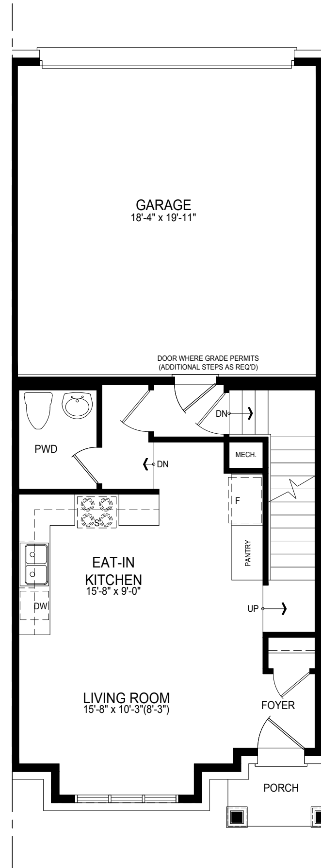
Main Floor Elev. A
