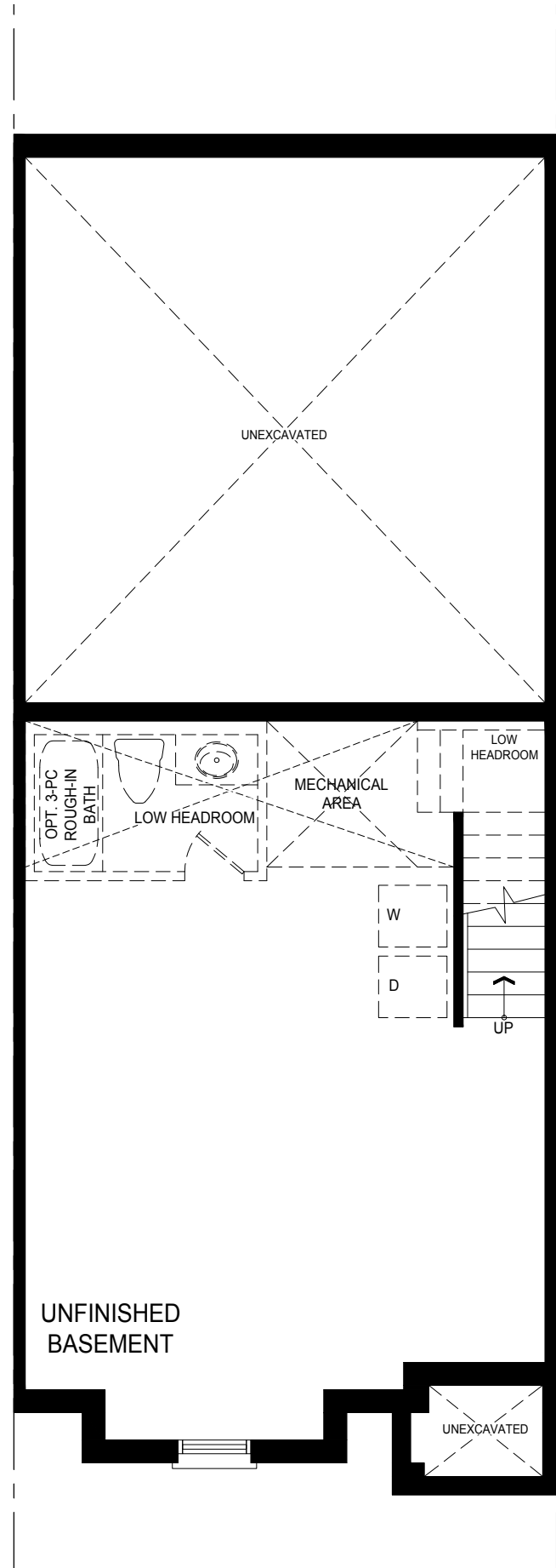
Basement Elev. A
