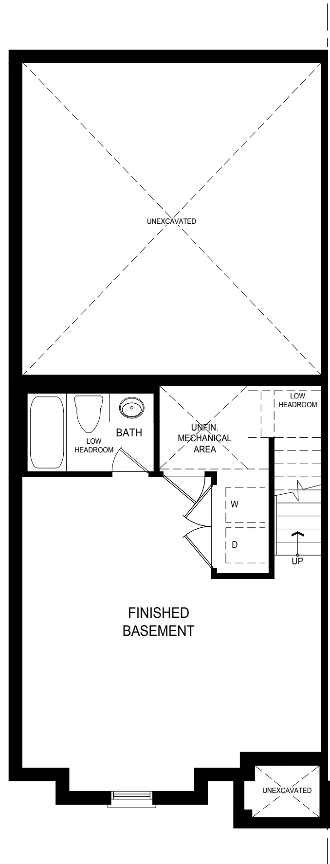
Basement Elev. A
