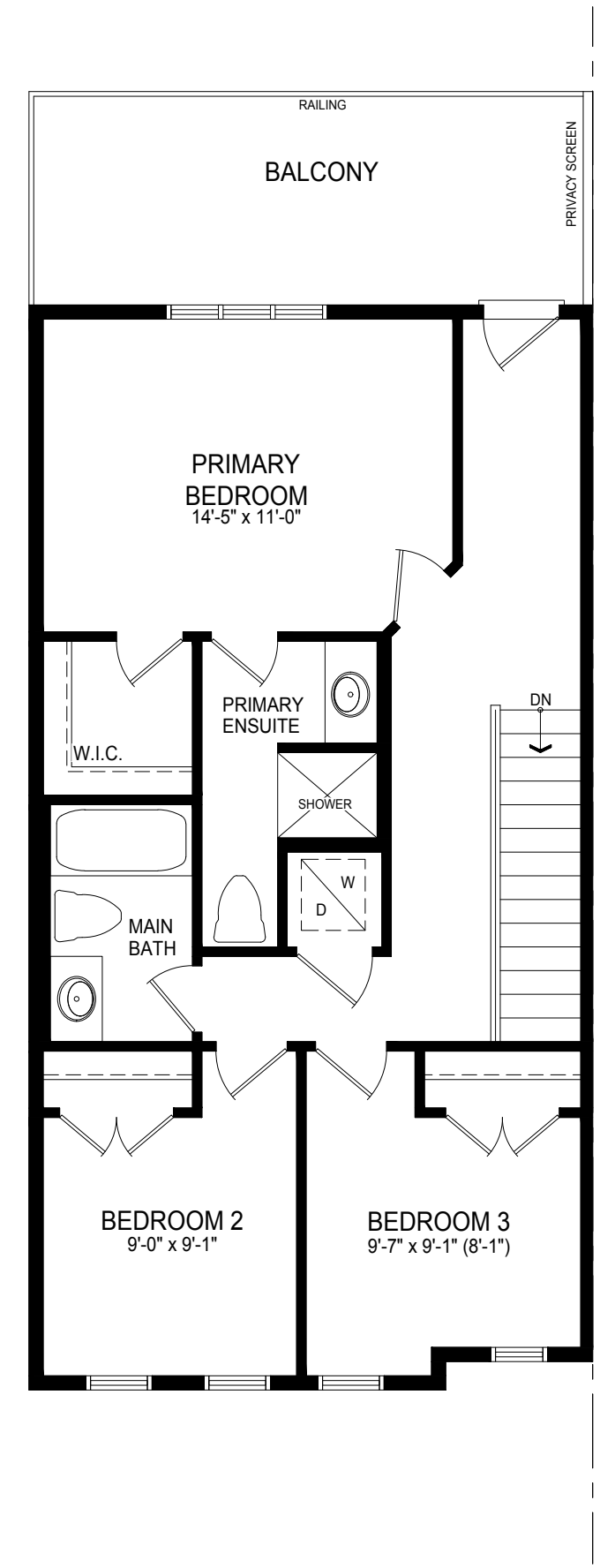
Upper Floor Elev. A
