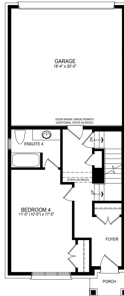
Modified Opt. Ground Floor Elev. A1
