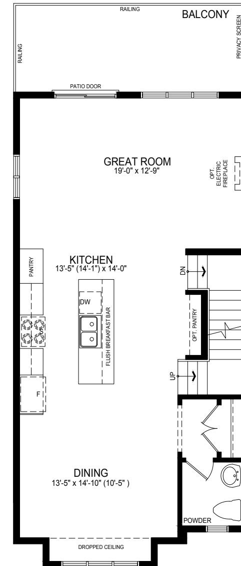
Modified Main Floor Elev. A1
