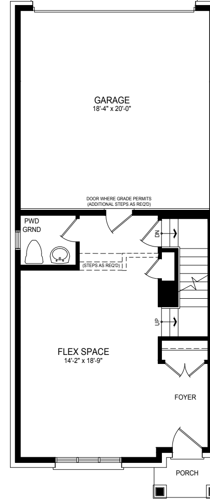
Modified Ground Floor Elev. A1
