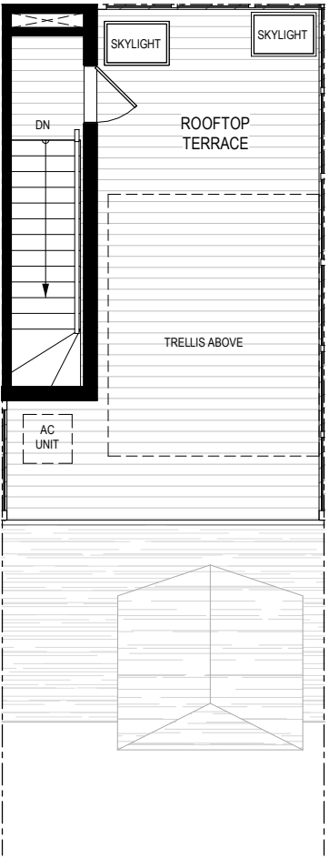
ROOFTOP TERRACE PLAN
