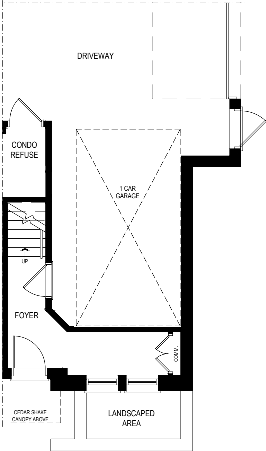
GROUND / BASEMENT FLOOR PLAN
